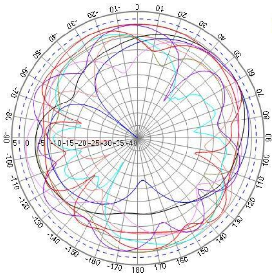
WIFI Antenna
