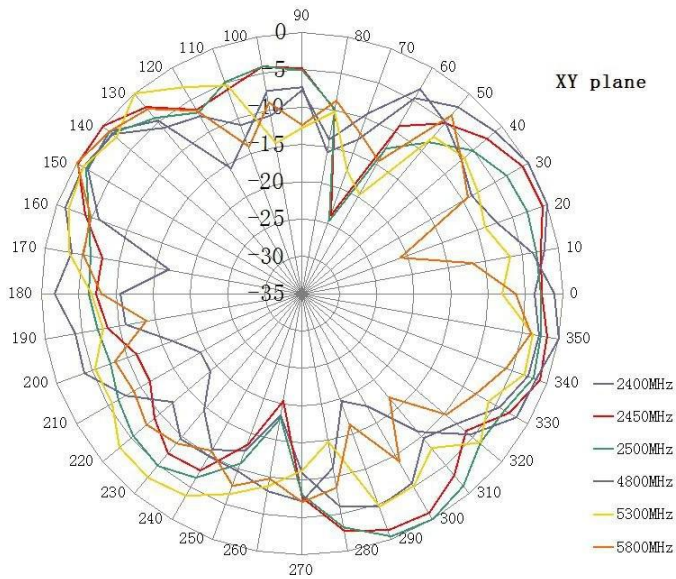
WIFI Antenna
