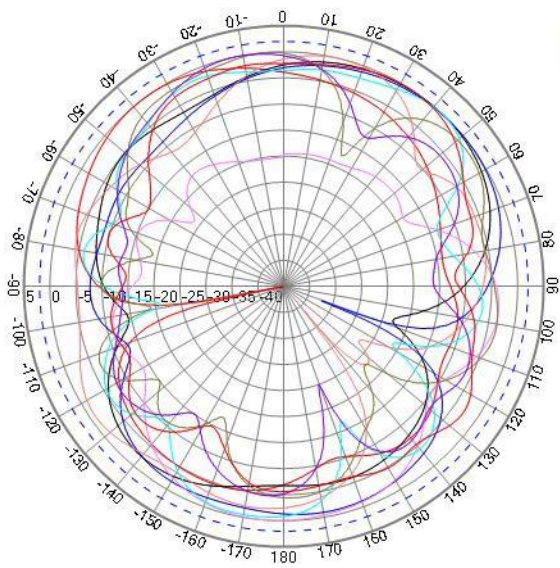
XZ PLANE
